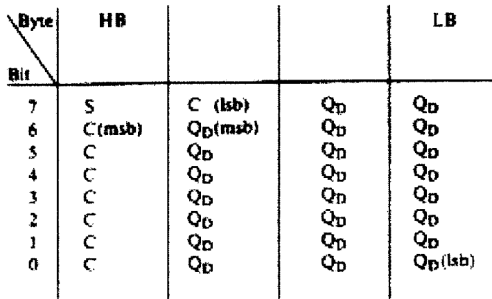
FIG. B-4. Description of one data sample in 32-bit floating-point format (S: sign bit, C: binary exponent bit, Q D = data bit, HB= high byte, LB = low byte (least significant bits), msb = most significant bit, lsb = least significant bit). Note that the order of the 4 bytes (i.e., LB first or HB first) is dependent on the specification of the first two bytes of the File Descriptor Block.
