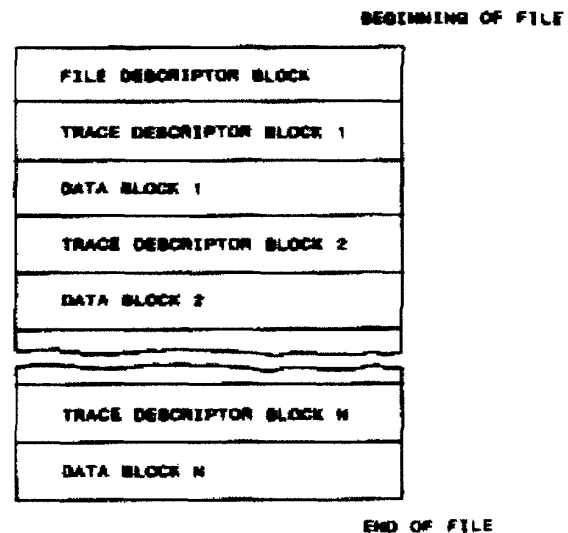
FIG. 1. File format
