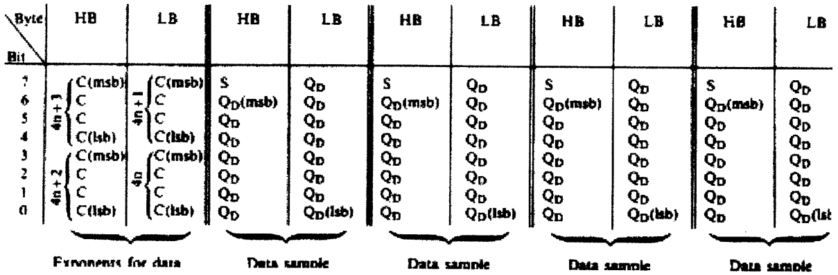
FIG. B-3. Description of four successive data samples in 32-bit floating point format (S = sign bit, C = binary exponent bit, Q D = data bit, HB = high byte, LB = low byte (least significant bits), msb = most significant bit, lsb = least significant bit). Note that the order of each group of two bytes (i.e., LB first or HB first) is dependent on the specification of the first two bytes of the File Descriptor Block.
