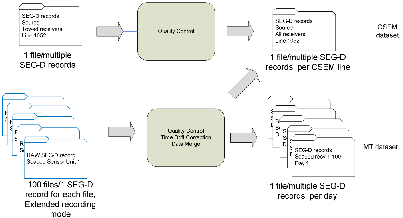
Summary of data flow - extended recording mode records are blue, normal recording mode records are black.
