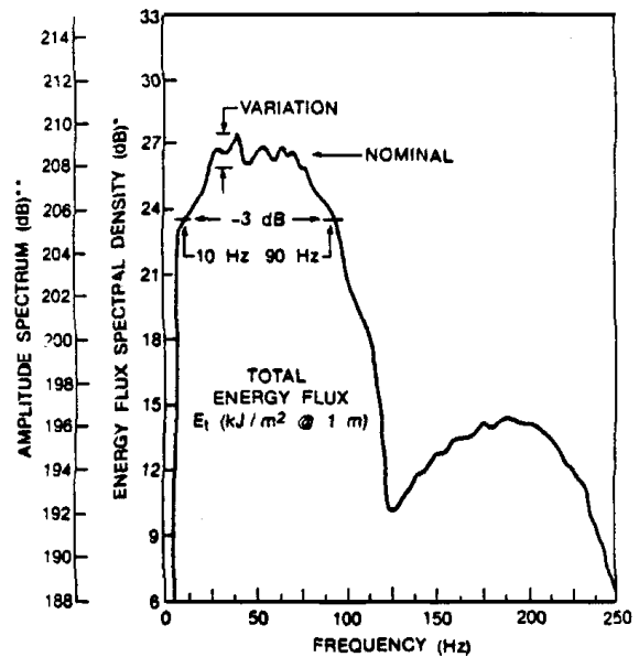
FIG. 2. Energy flux spectral density.
