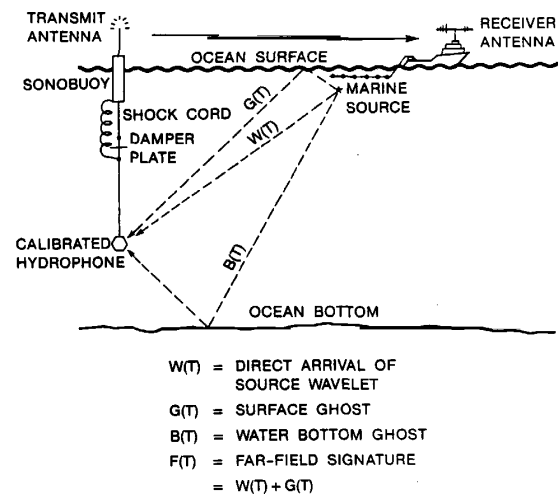
FIG. 3. Sonobuoy acquisition system.
