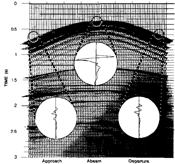
FIG. A-6. Results of the dynamic source test.
