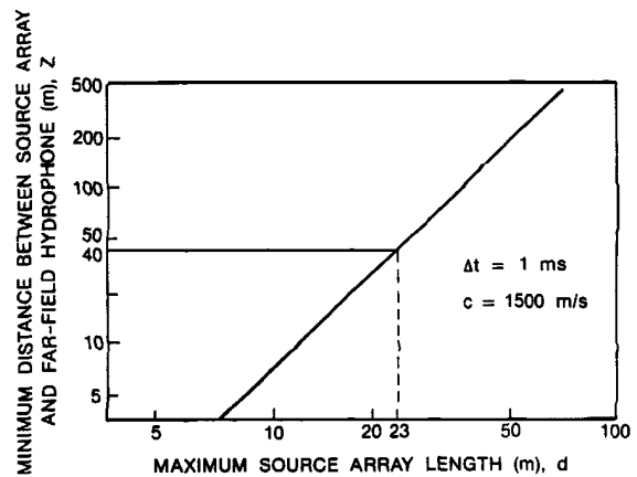
FIG. A-4. Minimum distance between the source array and the far-field hydrophone as a function of the length of the source array.
