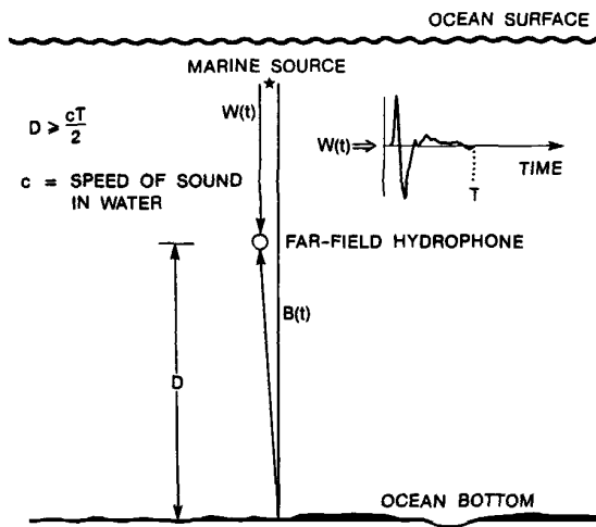
FIG. A-1. Minimum distance between the far-field hydrophone and the ocean bottom.
