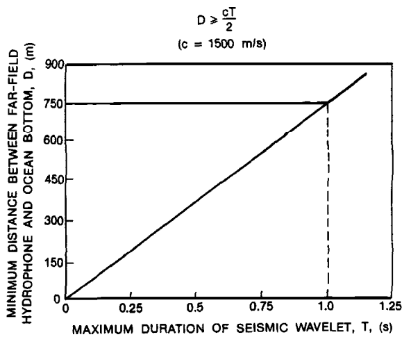
FIG. A-2. Minimum distance between the far-field hydrophone and the ocean bottom as a function of the seismic wavelet's duration.
