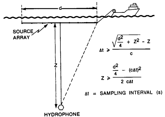
FIG. A-3. Minimum distance between the source array and the far-field hydrophone.
